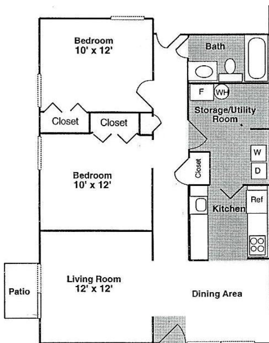
Floor Plan C 910 sq. ft.
